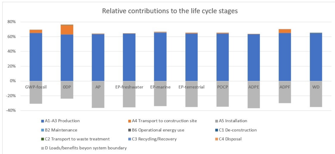
Figure 1: Environmental impacts of lock cylinders along its life cycle
