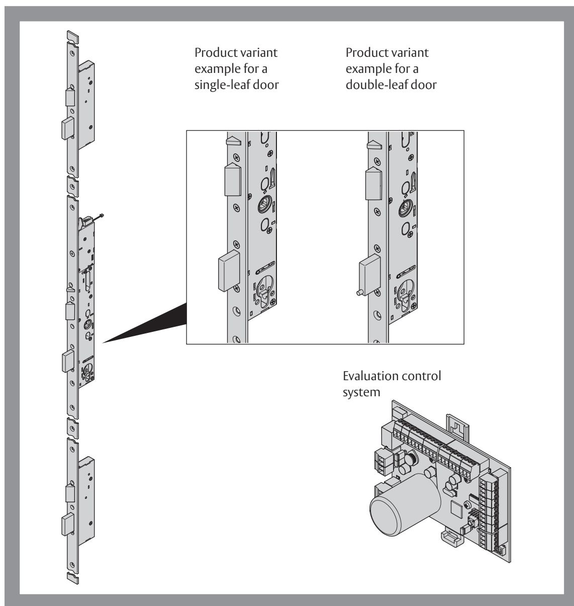
Fig. 1: mFlipLock access/ e-access panic/security/ multipoint locking
