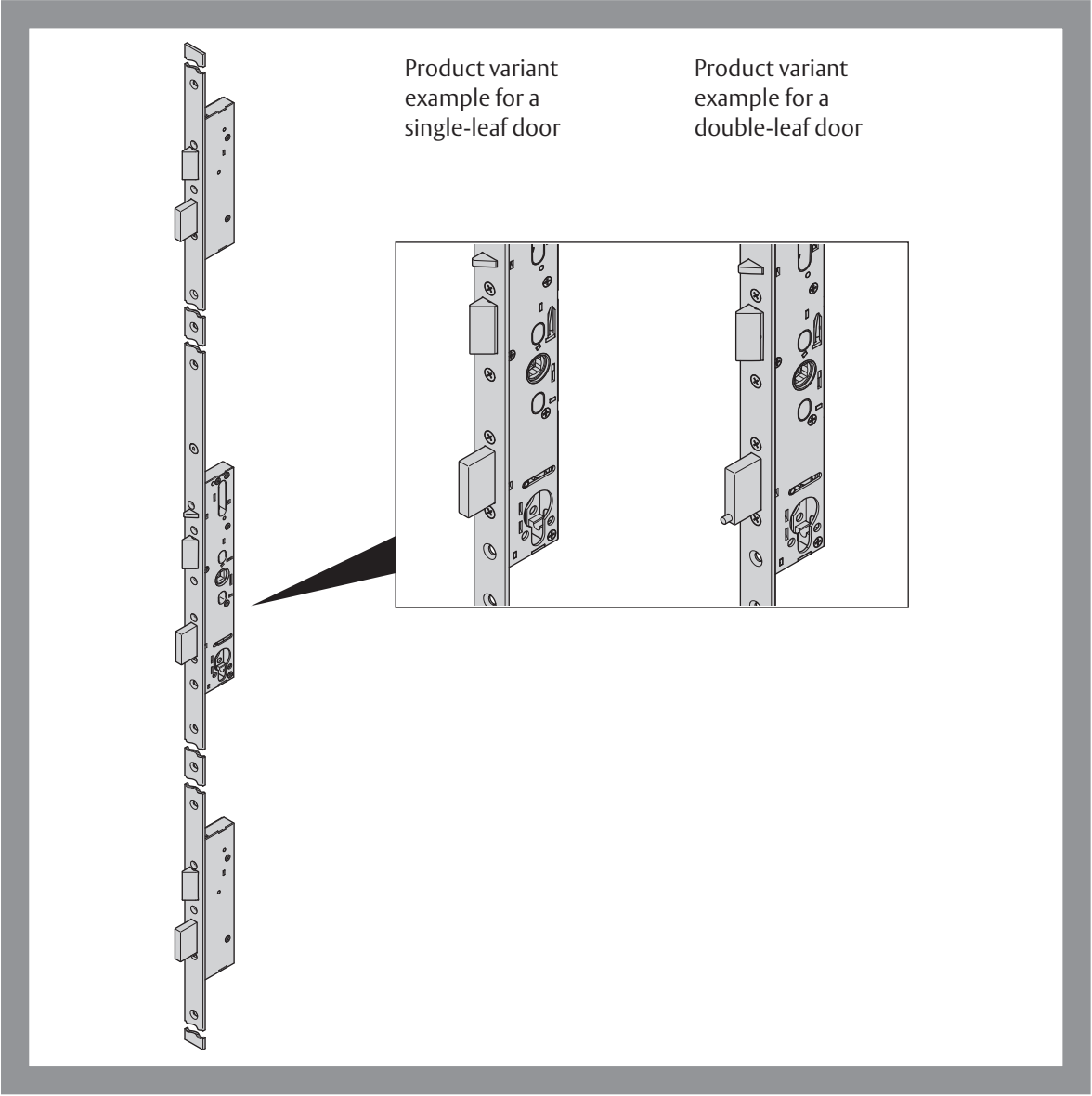
Fig. 1: Panic/security/ multipoint lock mFlipLock standard
