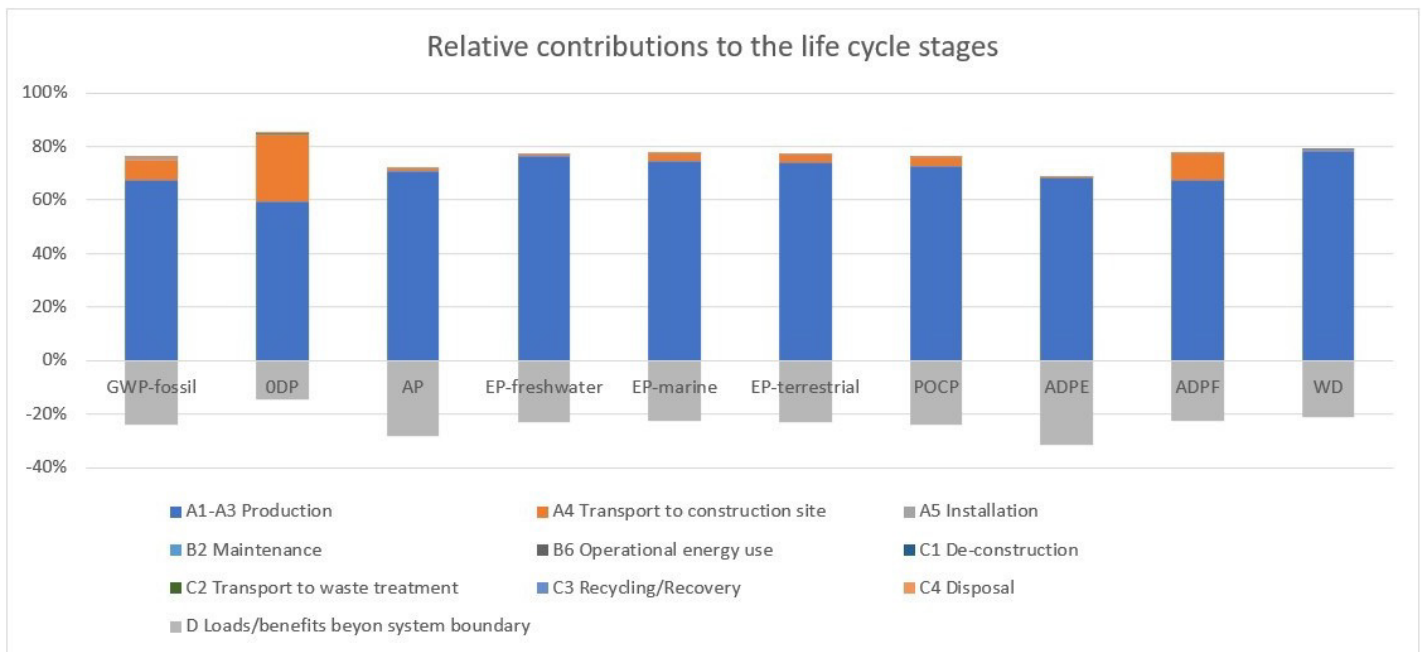
Figure 1: Environmental impacts of locks along its life cycle (impacts from production modules A1-A3 = 100 %)
