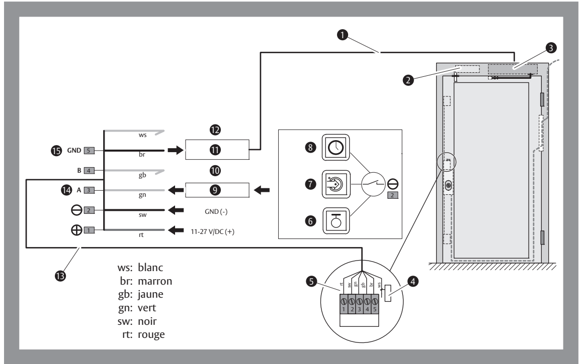
Schéma de raccordement sFlipLock 15544PE-SV drive
