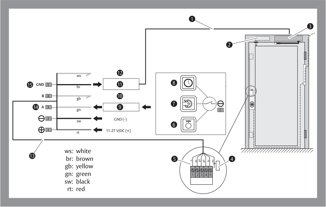
Fig. 11: Connection schematic for sFlipLock 16546PB-SV drive
