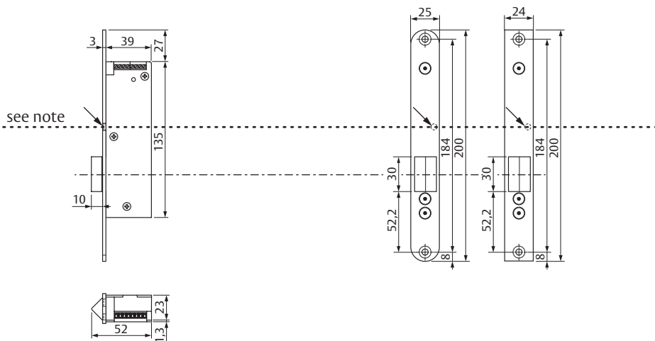
Escape door locking system 352M
