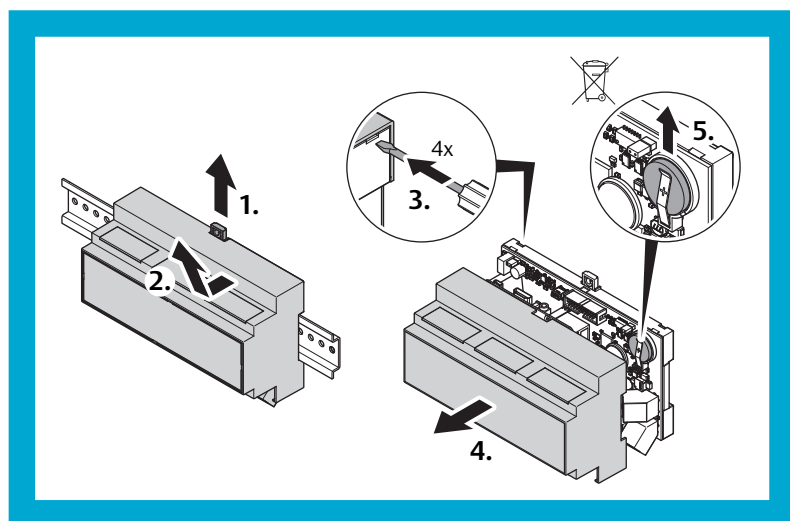
Fig. 7: Remove battery
