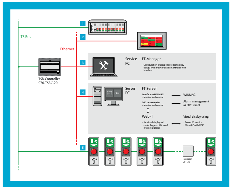
Fig. 3: Network structure
