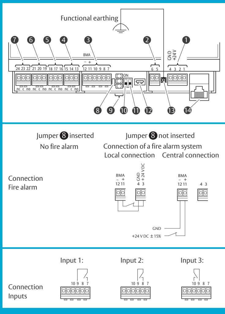
Fig. 2: Terminal strip
