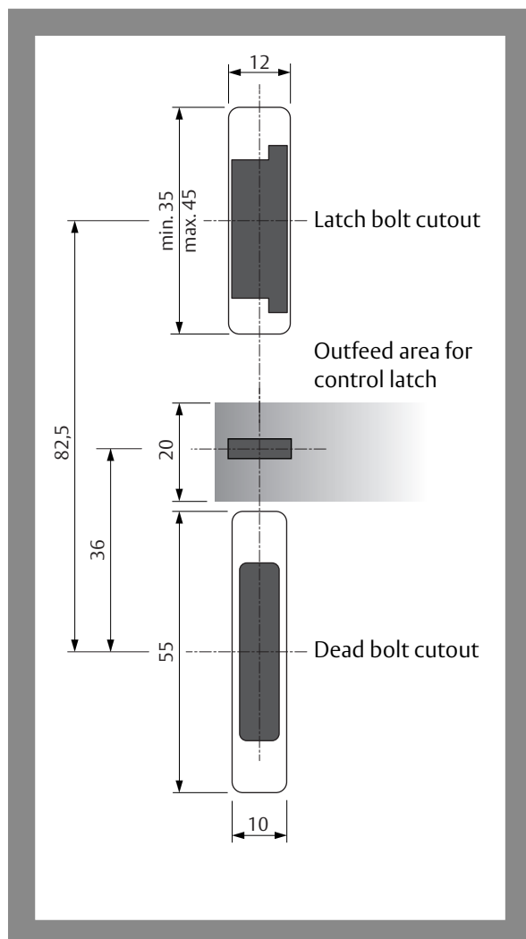
Pic. 9: Measurements for finishing customer-provi- ded striking plates
