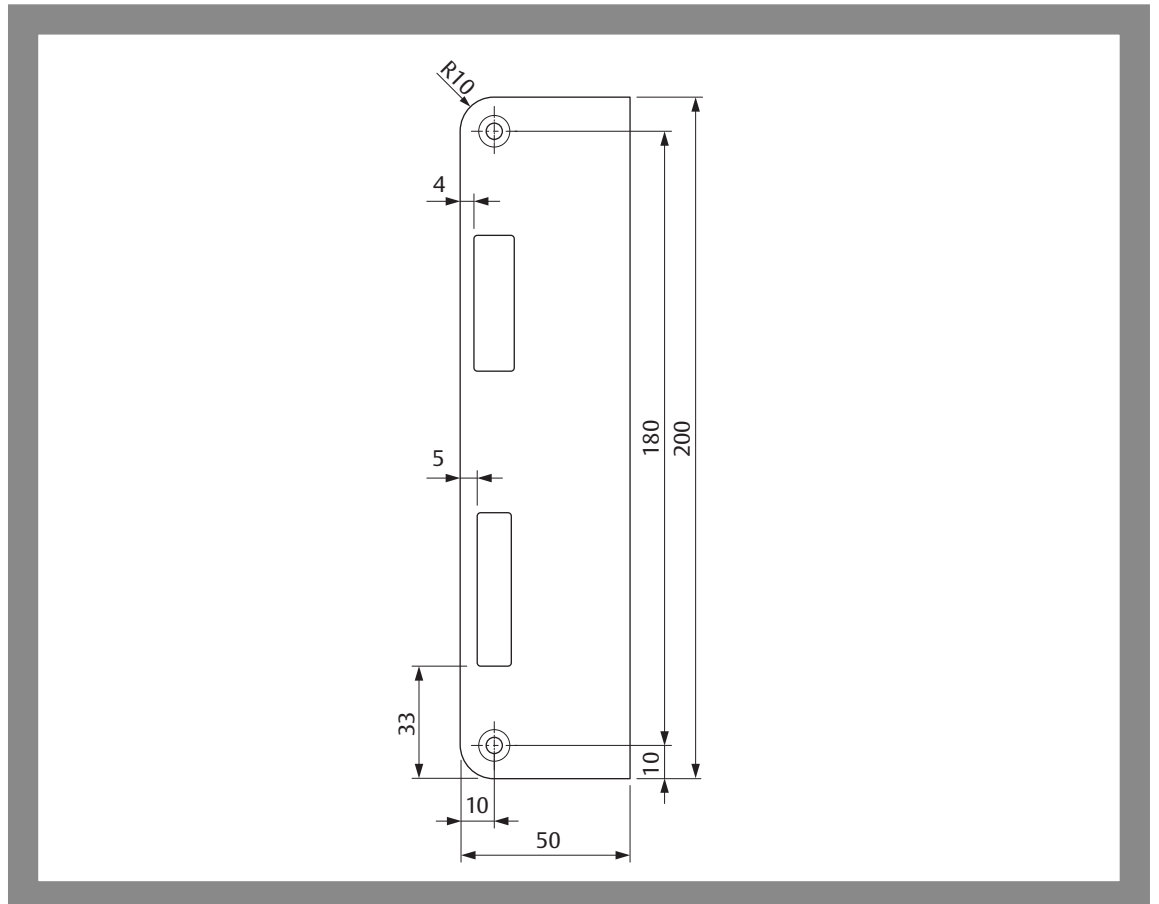
Pic. 14: Flanged striking plate
