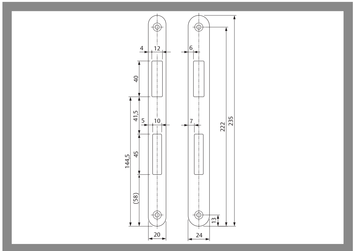
Pic. 11: Flat striking plate, various widths
