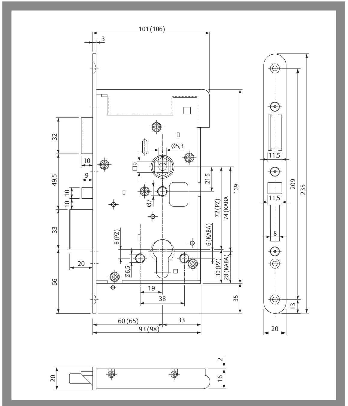
Pic. 10: Dimensions of the solid leaf security lock 309
