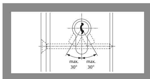
Pic. 8: Key withdrawal position
