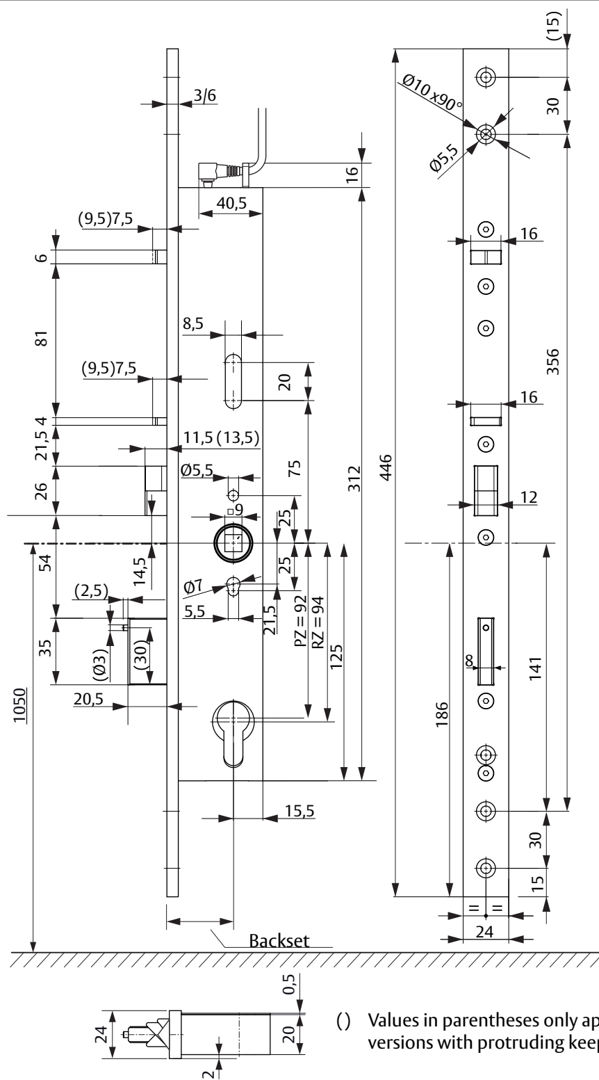
Fig. 17: Motorised security lock 509N dimensions
