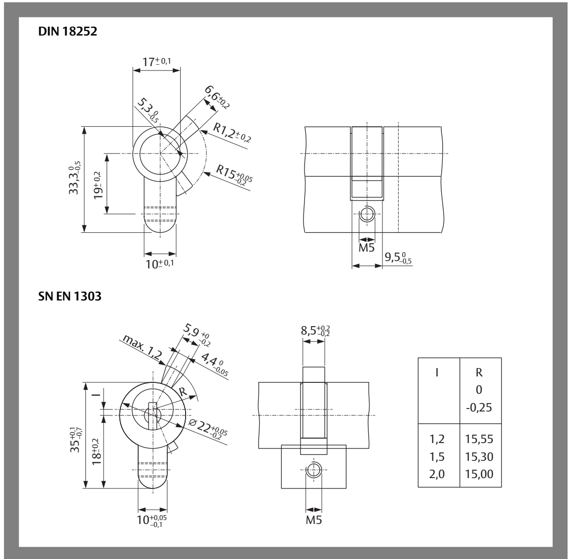
Fig. 18: Lock cylinder dimensions according to DIN 18252 or SN EN 1303
