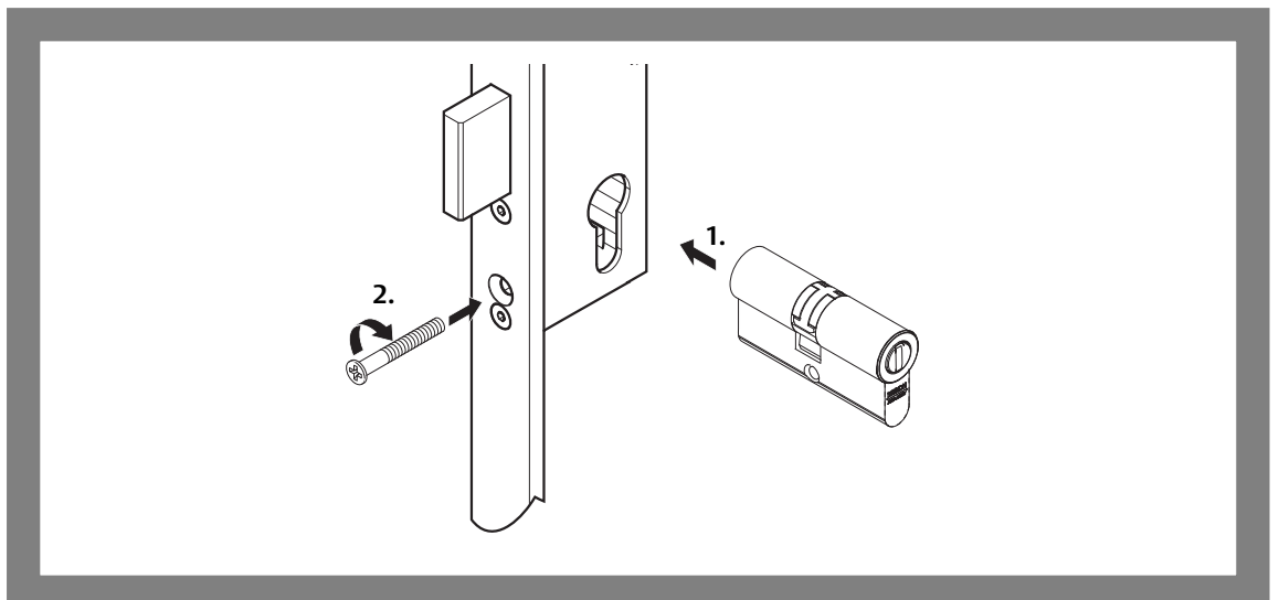
Fig. 13: Install a profile cylinder
