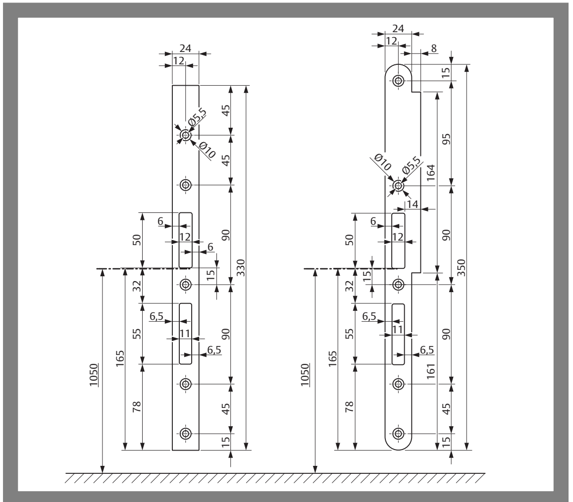
Fig. 19: Striking plates
