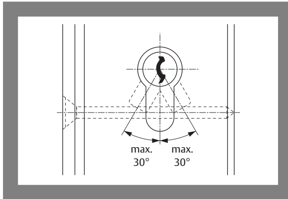
Fig. 12: Key withdrawal position
