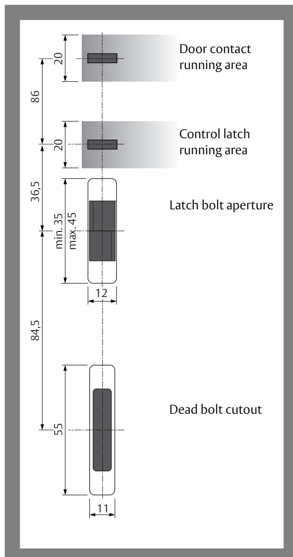
Fig. 16: Measurements for production of customer- provided striking plates
