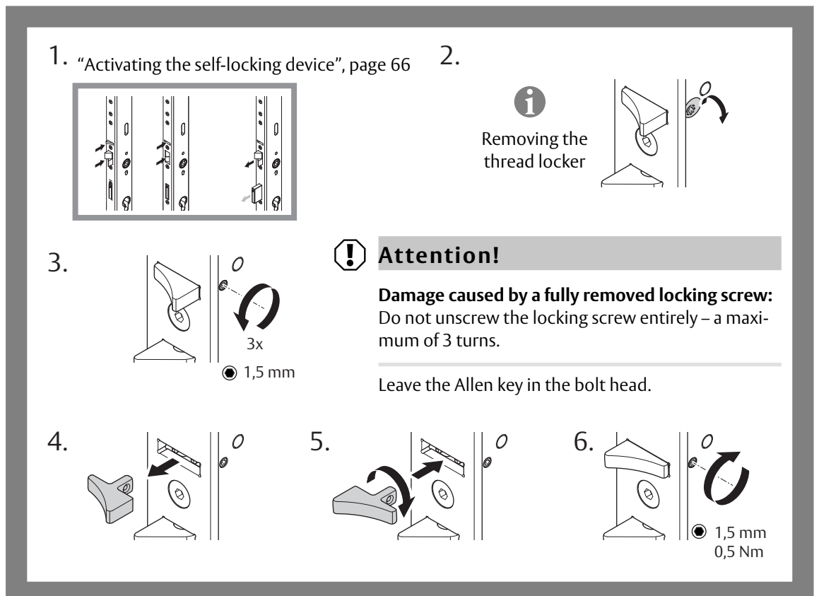
Fig. 9: Rotating the control latch
